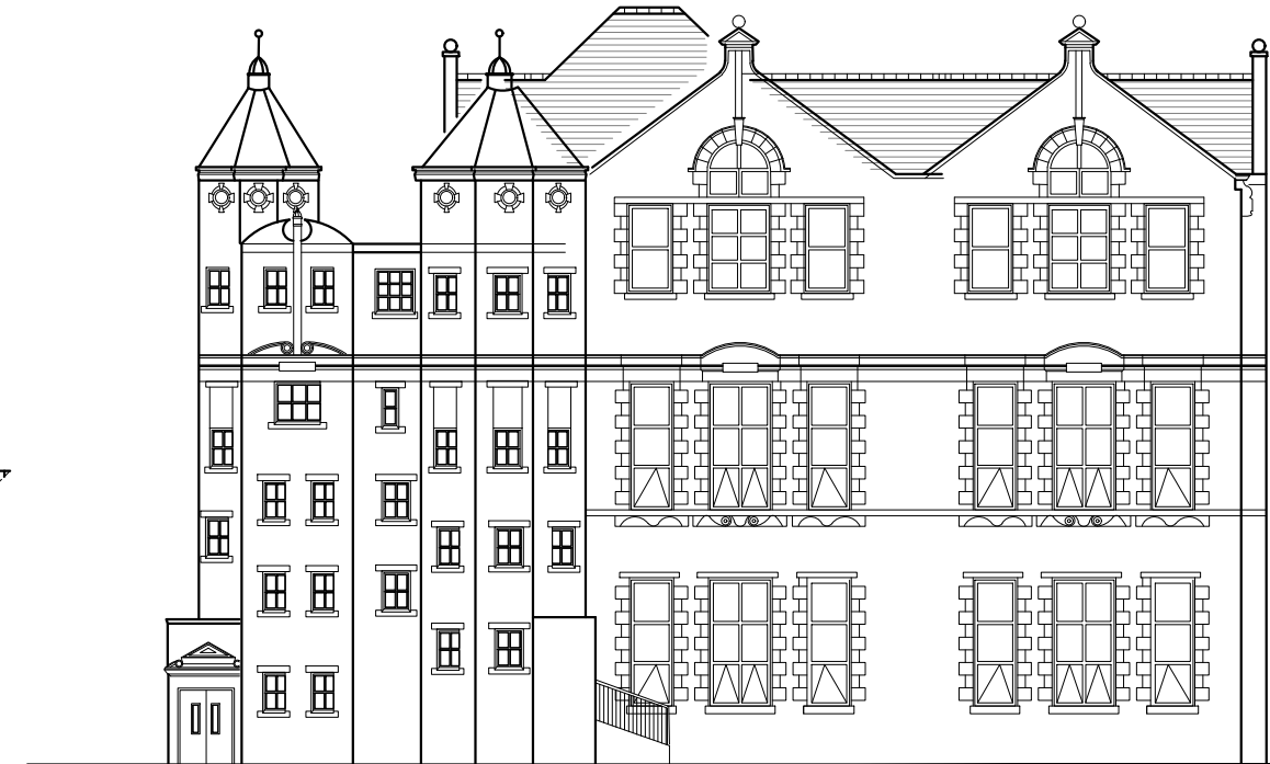
EXISTING SIDE ELEVATION SCALE: 1/200 @A3
